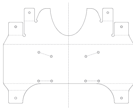
Brace protector
